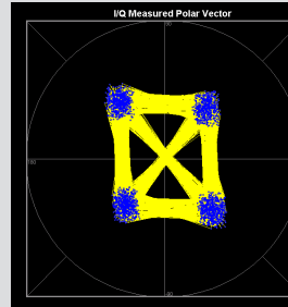
Calibrated AWGN to simulation a noisy environment.
