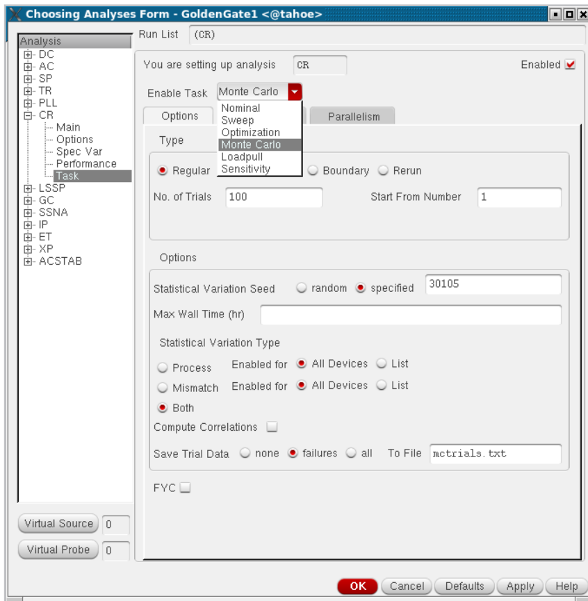
Figure 5. The Choosing Analyses Form simplifies the setup of advanced analyses. The Task field provides access to a variety of multiple-run simulations including Monte Carlo analysis. Fast Yield Contributor (FYC) analysis is a unique capability which enables very fast computation of device-level contributions within Monte Carlo analysis.
