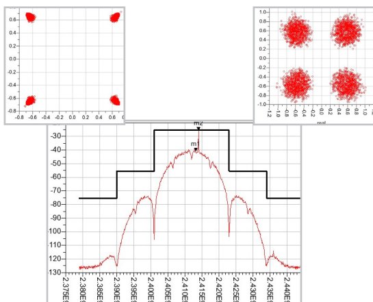
Figure 13. GoldenGate lets designers investigate the impact of blockers on system-level metrics directly in Virtuoso.
