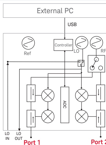
Figure 1. P937XA USB Vector Network Analyzer block diagram
