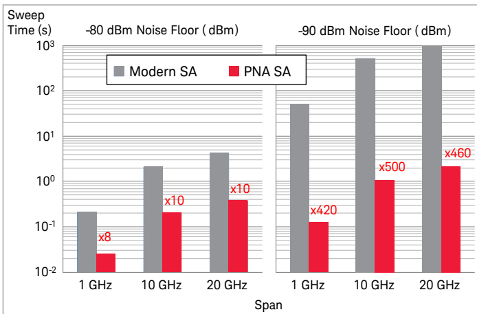
Sweep time versus span with 12 GHz center frequency for -80 dBm and -90 dBm noise floor. The receiver attenuator is set to avoid compression with a +10 dBm signal.
