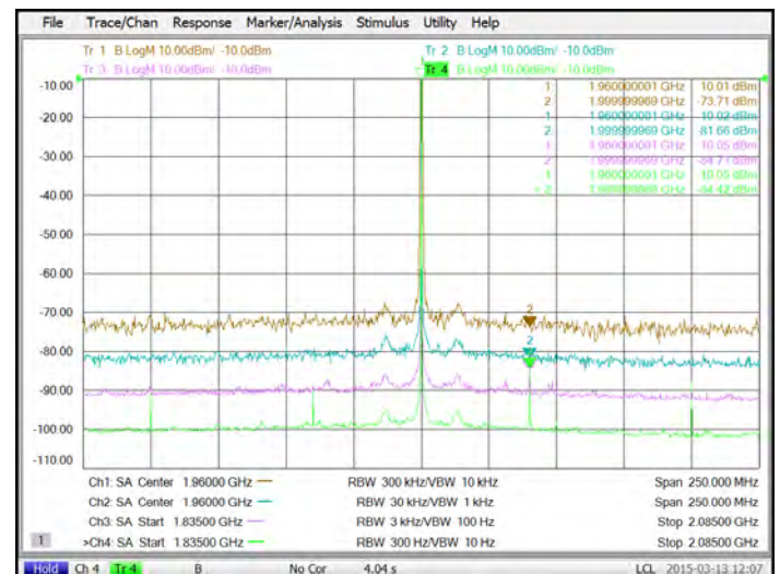
Above plot shows -84 dBm spurious measurements in the presence of a +10 dBm signal, with (from top to bottom) approximate S/N (at RBW) of 80 dB (300 kHz), 90 dB (30 kHz), 100 dB (3 kHz), and 110 dB (300 Hz)
