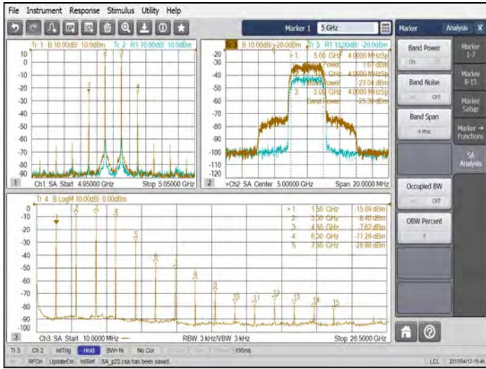
Spectrum analyzer option adds fast spur search capability to the PNA-X, replacing a standalone spectrum analyzer and switch matrix in component-characterization test systems.
