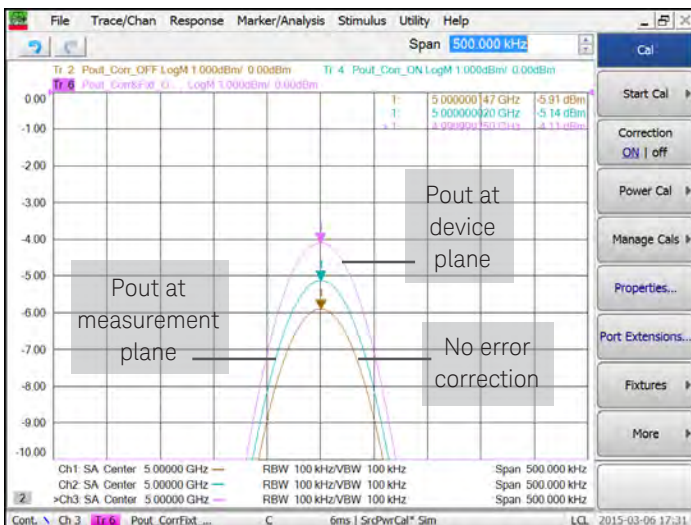
VNA calibration and fixture de-embedding remove cable and fixture effects and correct receiver response errors, providing calibrated in-fixture spectrum analysis.
