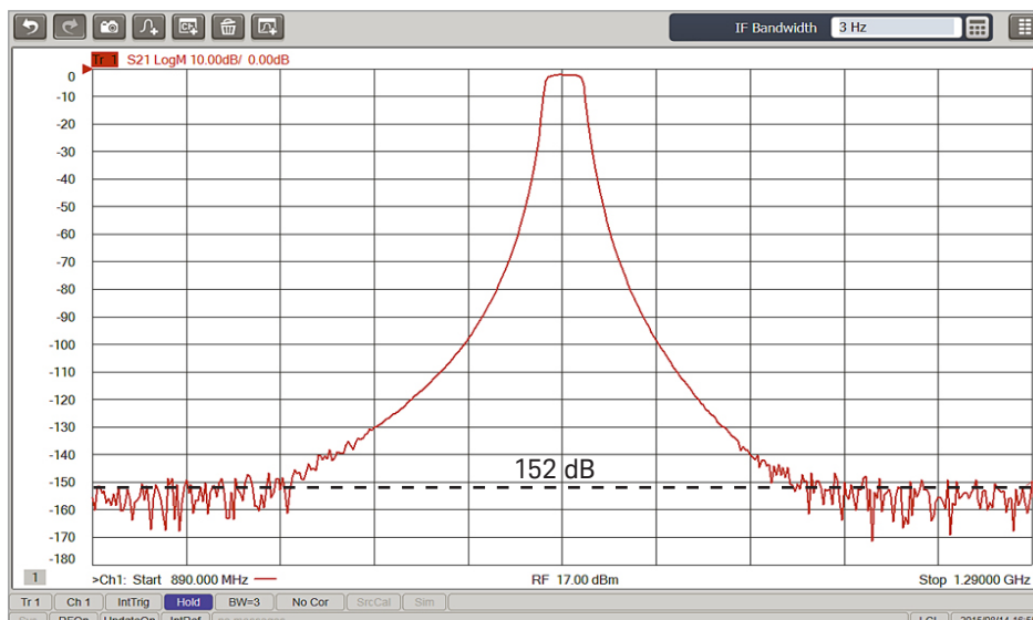
Figure 1. Wide dynamic range (IFBW = 3 Hz)
