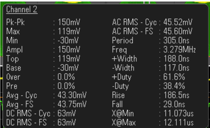
Snapshot of all 24 measurements being taken simultaneously.
